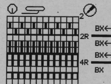
Diagram 2 for 3 colour Fairisle TECH 197
